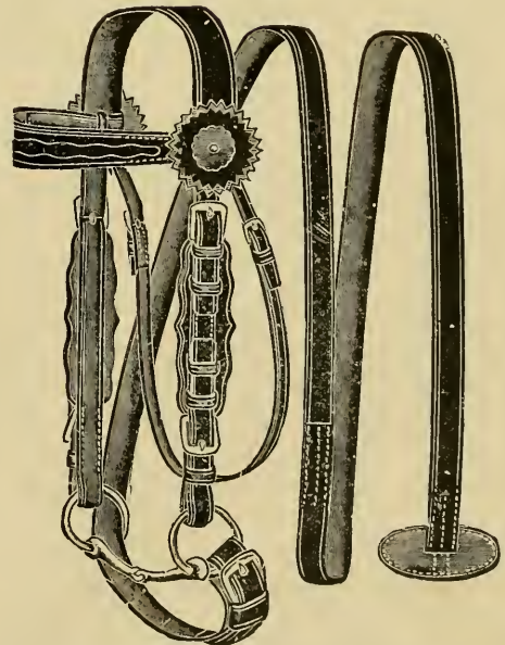
No. 35. FANCY STALLION BRIDLE—Black leather, solid crown, \frac{7}{8} inch fancy cheeks, 1 inch lead, fancy leather front, nickel or brass trimmings, extra heavy straight mouth ring bit. (Wrong bit is shown.)
